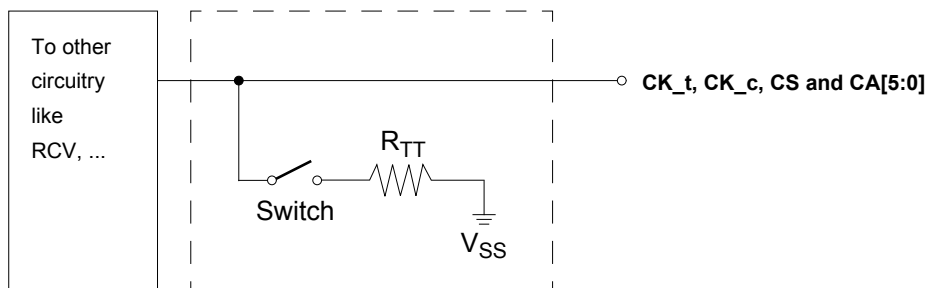
Figure 115: Functional Representation of CA ODT
