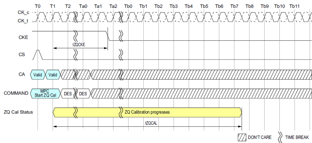
Figure 133: Multi purpose Command for Start ZQ Calibration to Power-Down Entry
