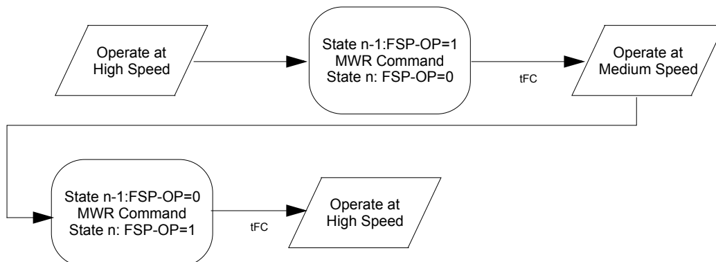
Figure 92: Switching Between Two Trained Frequency Set-Points
