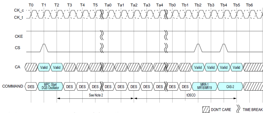
Figure 108: In case of DQS Interval Oscillator is stopped by DQS interval timer
