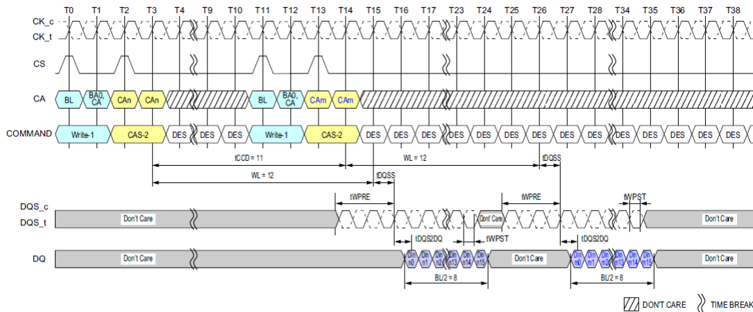
Figure 42: Consecutive Writes Operation: t_{CCD} = \text{Min} + 3, 0.5nCK Postamble
