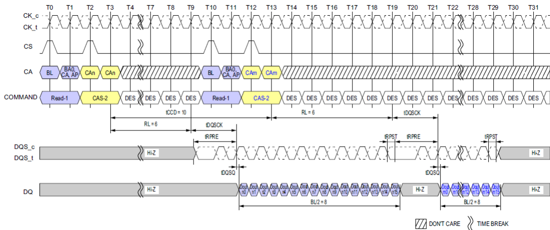
Figure 28: Consecutive Reads Operation: t_{CCD} = \text{Min} + 2 , Preamble = Toggle, 0.5nCK Postamble
