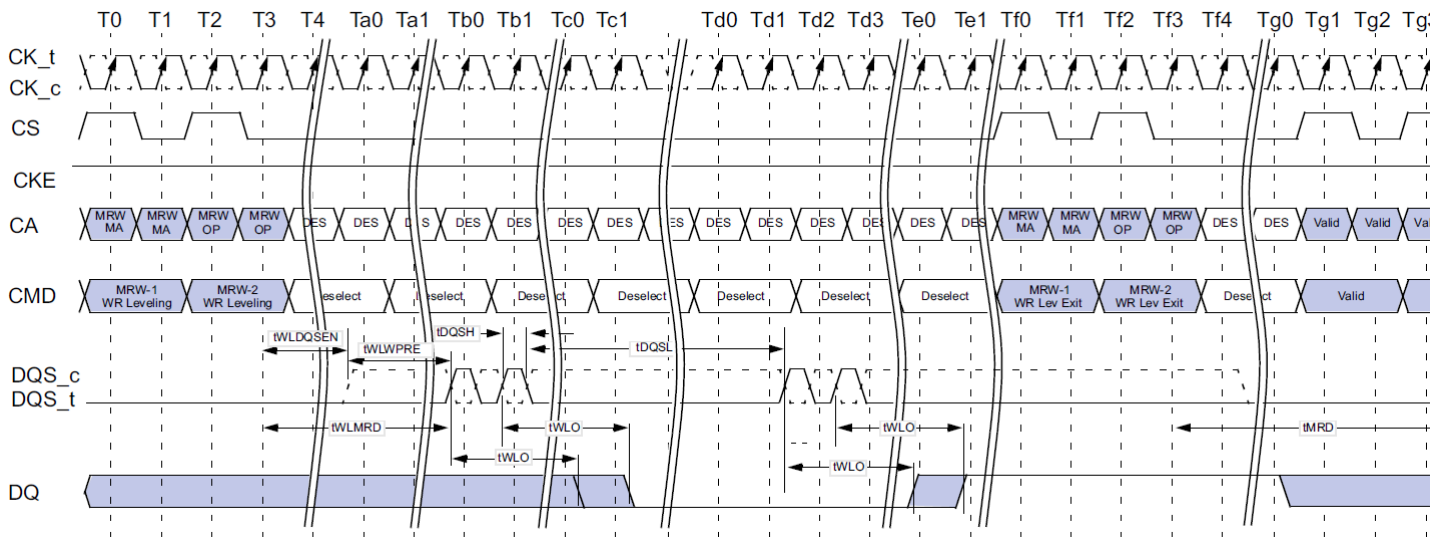
Figure 94: Write Leveling Timing, t_{DQSL(max)}
