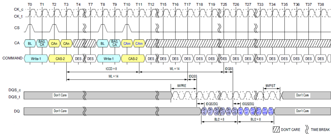
Figure 37: Seamless Writes Operation: t_{CCD} = \text{Min}, 1.5nCK Postamble
