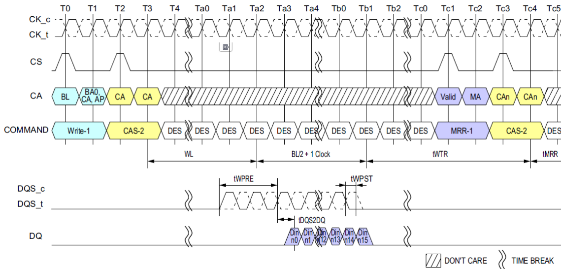
Figure 67: Write to MRR Timing
