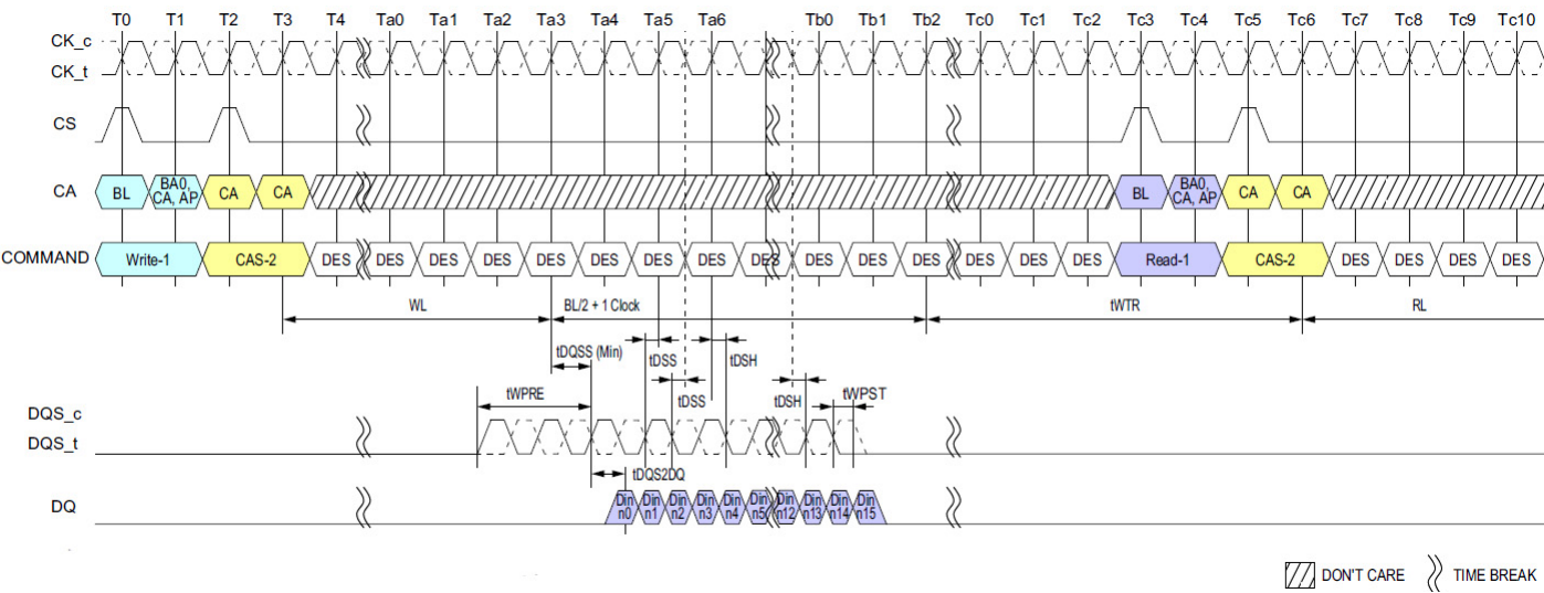
Figure 18: Burst Write Followed By Burst Read
