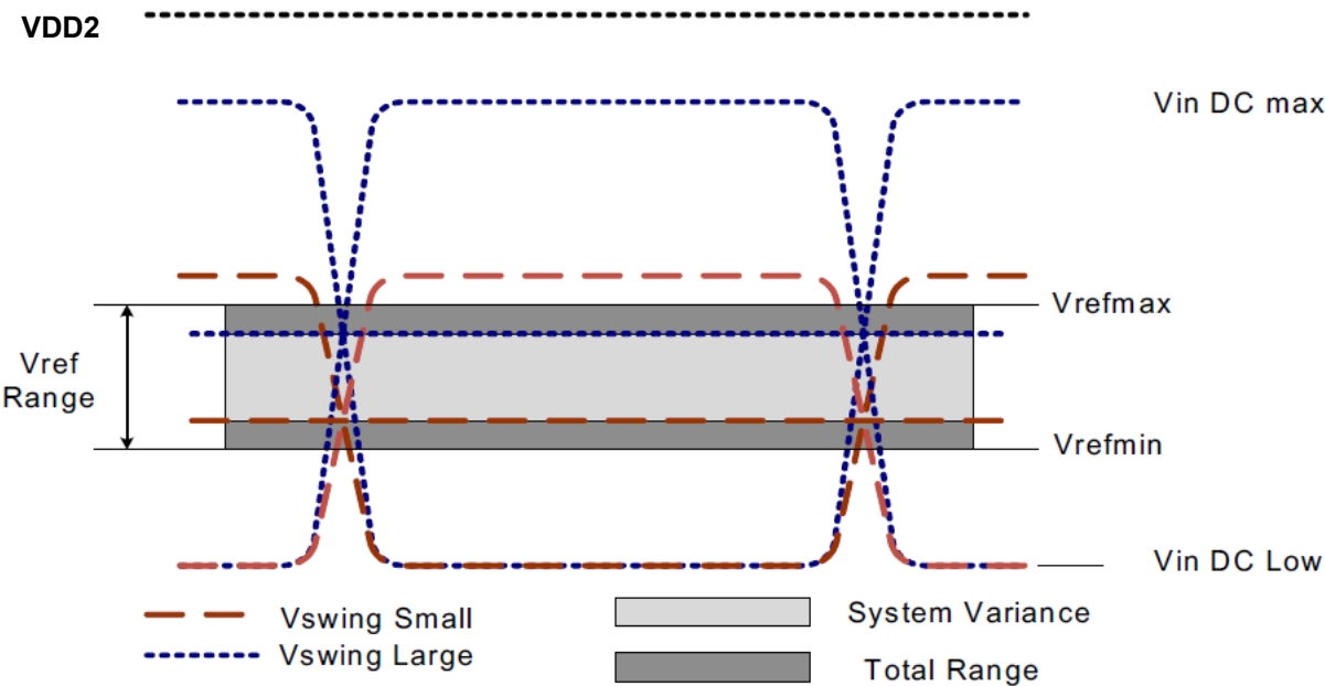
Figure 72: Vref operating range(Vrefmin, Vrefmax)
