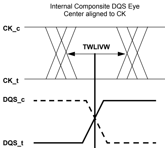
Figure 97: DQS_t/DQS_c to CK_t/CK_c timings at the DRAM pins referenced from the internal latch
