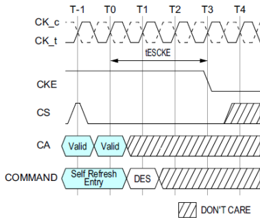
Figure 17. tESCKE Timing
