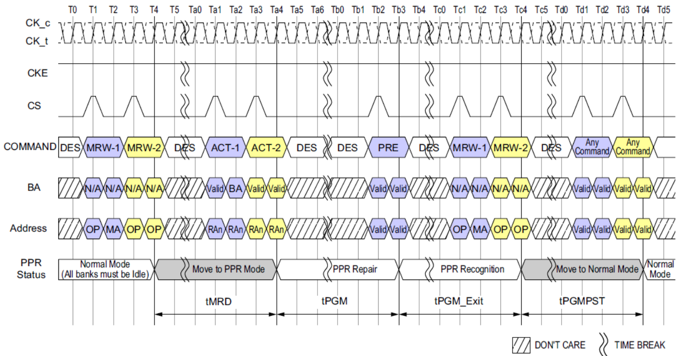
Figure 134: PPR Timing
