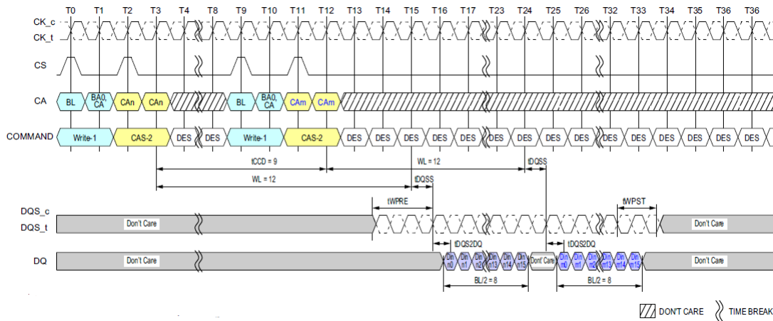
Figure 39: Consecutive Writes Operation: t_{CCD} = \text{Min} + 1, 1.5nCK Postamble
