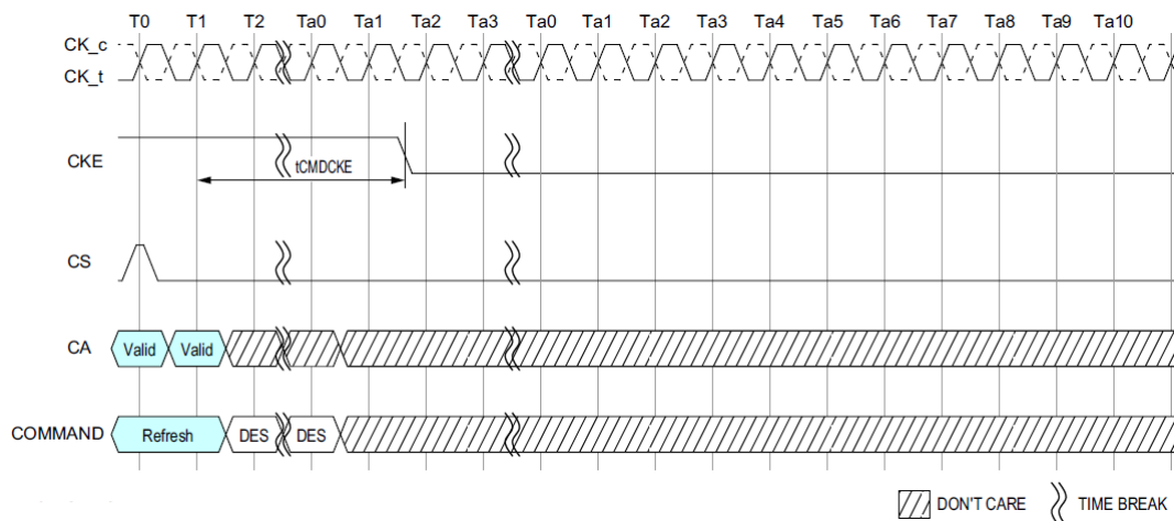
Figure 128: Refresh entry to Power-Down Entry
