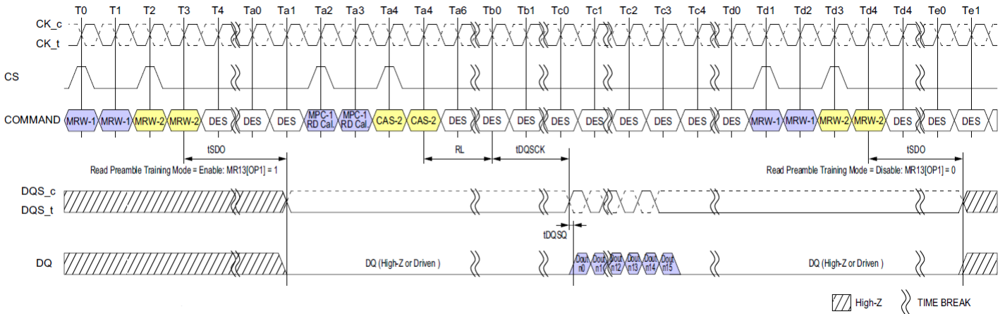
Figure 109: Read Preamble Training
