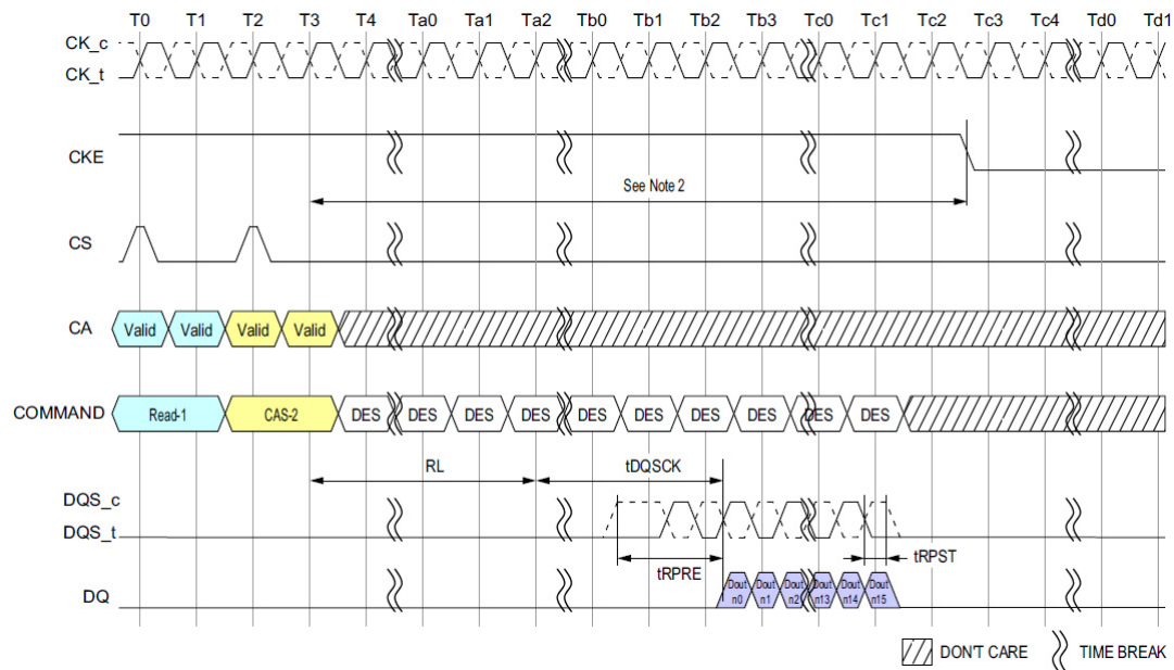
Figure 125: Read and Read with Auto Precharge to Power-Down Entry
