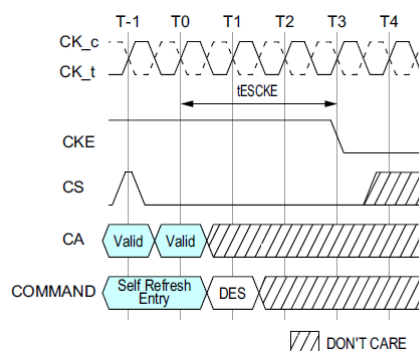
Figure 62: t_{ESCKE} Timing
