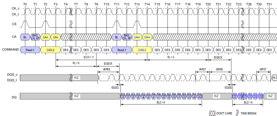
Figure 31: Consecutive Reads Operation: t_{CCD} = \text{Min} +3 , Preamble = Toggle, 1.5nCK Postamble
