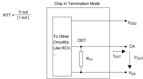
Figure 116: On Die Termination for CA
