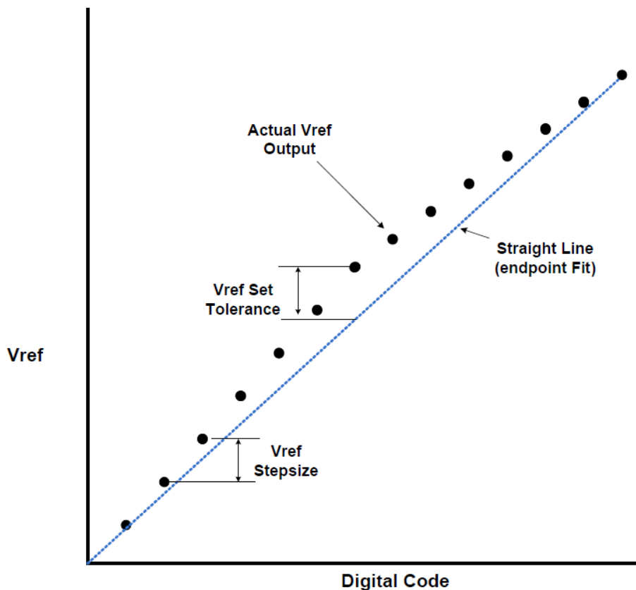
Figure 73: Example of Vref set tolerance(max case only shown) and stepsize
