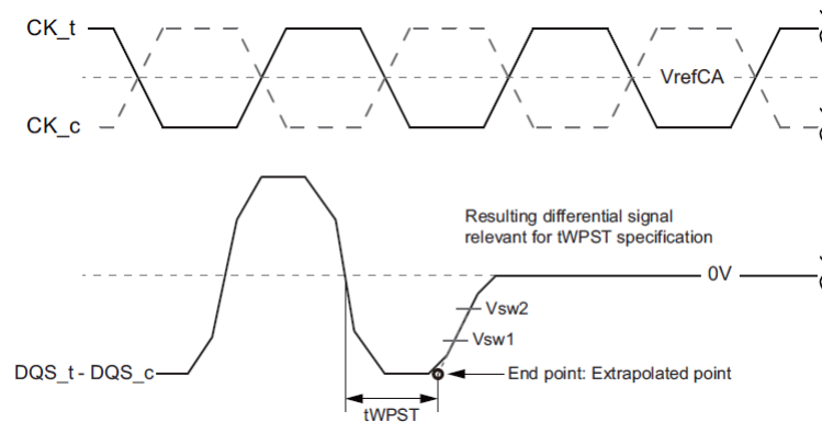
Figure 21: Method for calculating t_{WPST} transitions and endpoints
