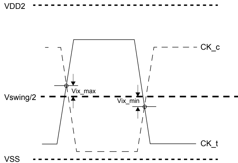
Figure 9. CK input Crosspoint voltage (Vix)
