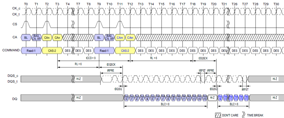
Figure 24: Consecutive Reads Operation: t_{CCD} = \text{Min} + 1 , Preamble = Toggle, 0.5nCK Postamble
