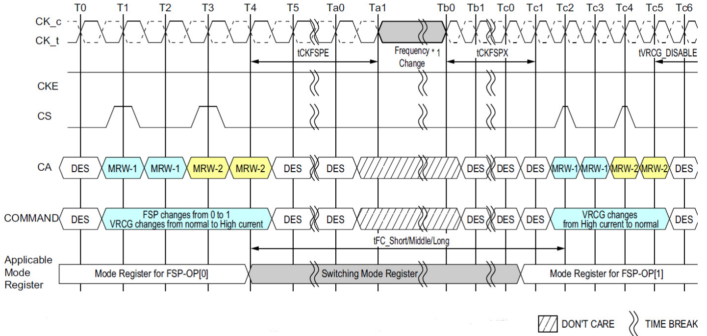
Figure 90: Frequency Set Point Switching Timing
