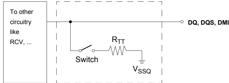
Figure 118: Functional Representation of ODT
