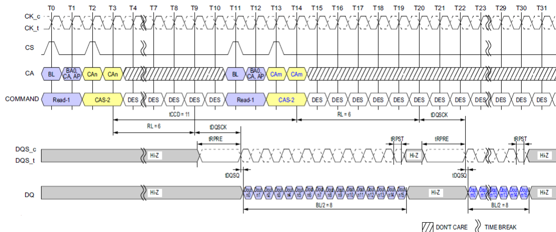
Figure 34: Consecutive Reads Operation: t_{CCD} = \text{Min} + 3 , Preamble = Static, 0.5nCK Postamble
