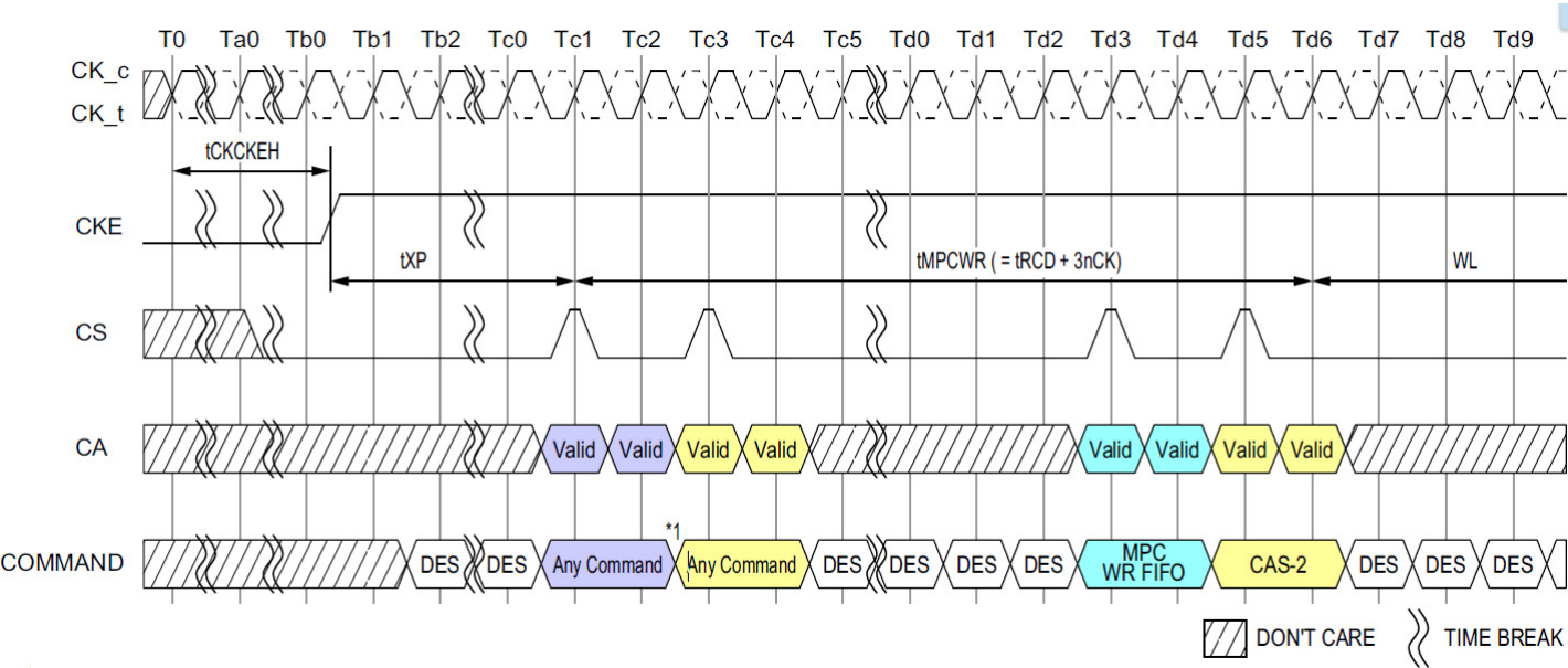
Figure 105: Power Down Exit to MPC [Write FIFO] Timing
