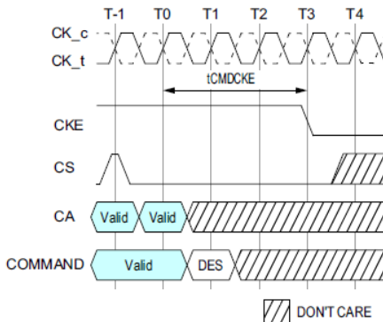
Figure 18. tCMDCKE Timing
