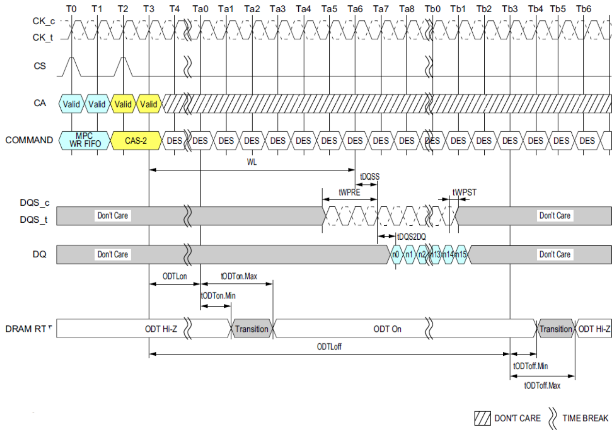
Figure 104: MPC [Write FIFO] with DQ ODT Timing
