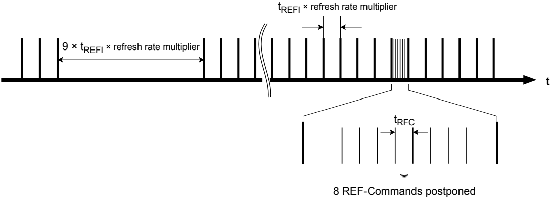
Figure 57: Postponing Refresh Commands (Example)
