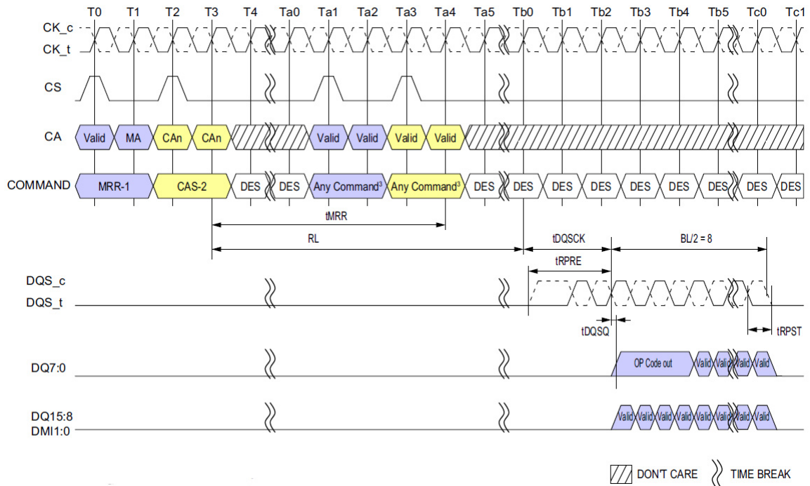
Figure 65: Mode Register Read Operation
