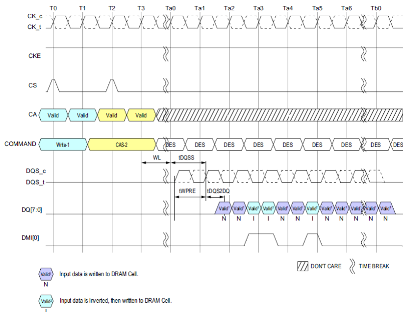
Figure 48: Write Command w/ Write DBI Enabled; DM Disabled
