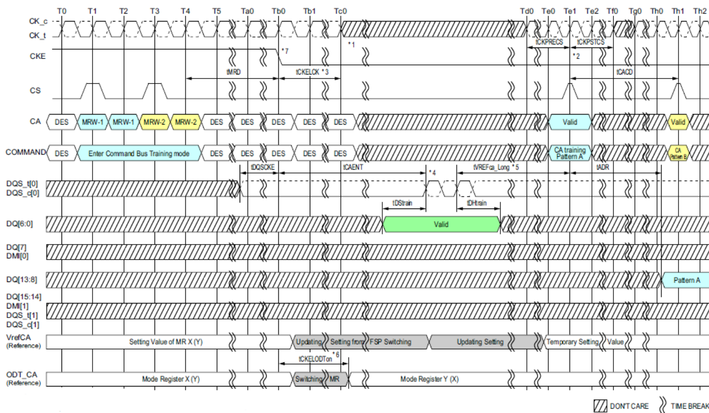
Figure 86: Entering Command Bus Training Mode and CA Training Pattern Input and Output with V_{REFCA} Value Update
