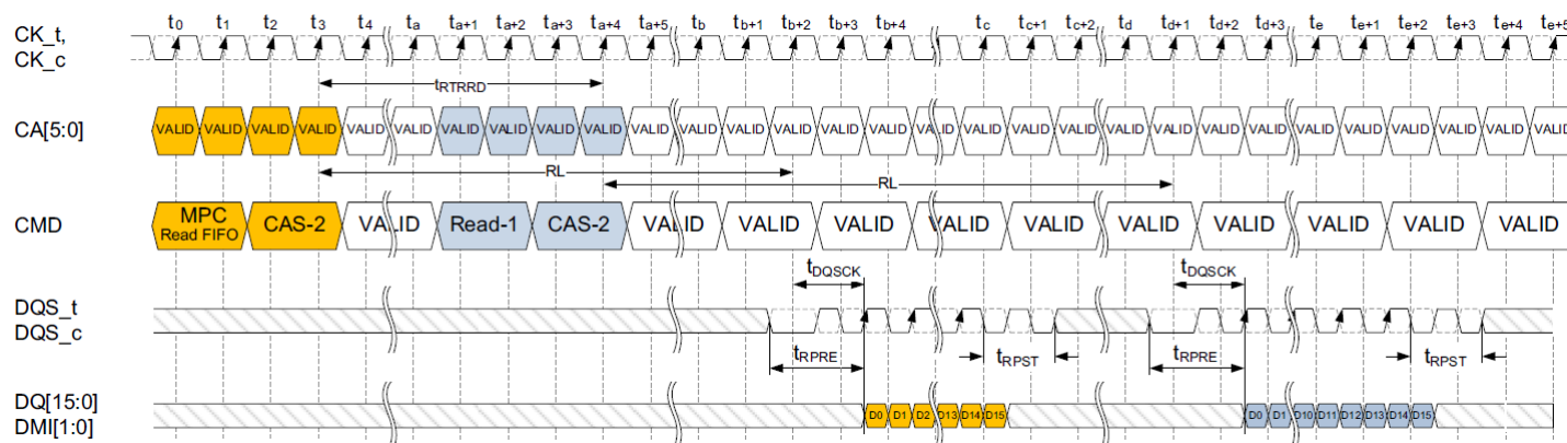
Figure 112: MPC [RD FIFO] Operation : tRPRE=toggling, tRPST=1.5nCK
