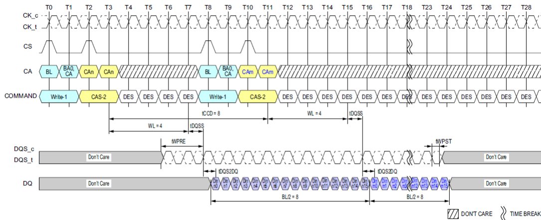
Figure 35: Seamless Writes Operation: t_{CCD} = \text{Min} , 0.5nCK Postamble
