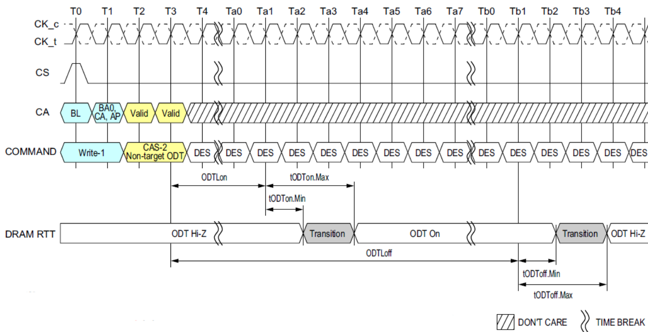
Figure 121: ODT Control on Non-target DRAM for Writes
