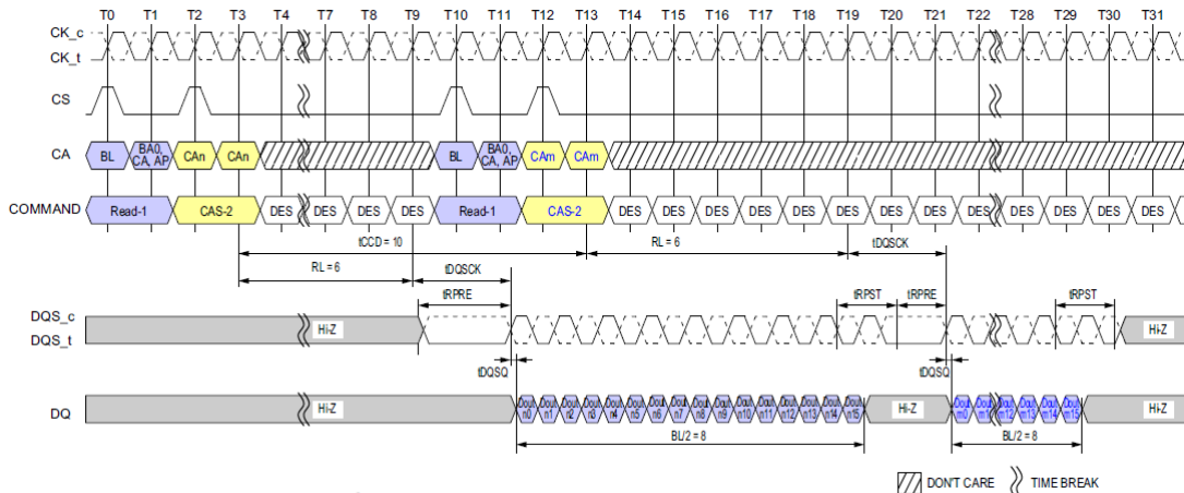
Figure 29: Consecutive Reads Operation: t_{CCD} = \text{Min} + 2 , Preamble = Static, 1.5nCK Postamble
