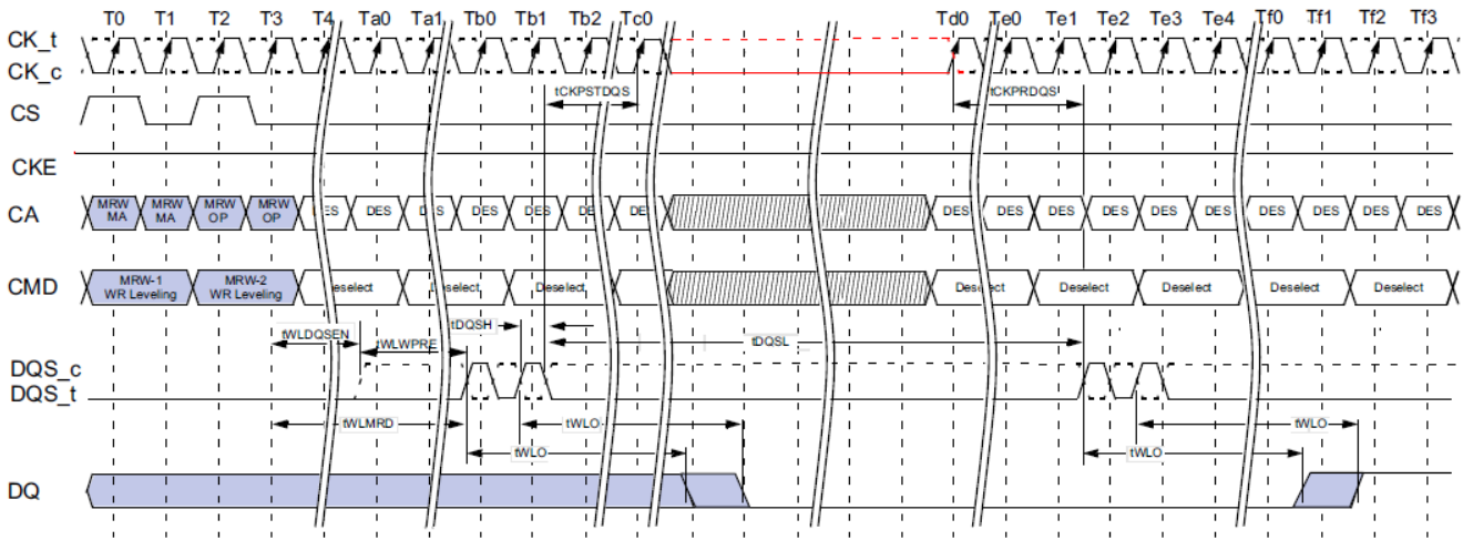
Figure 96: Clock Stop and Timing during Write Leveling
