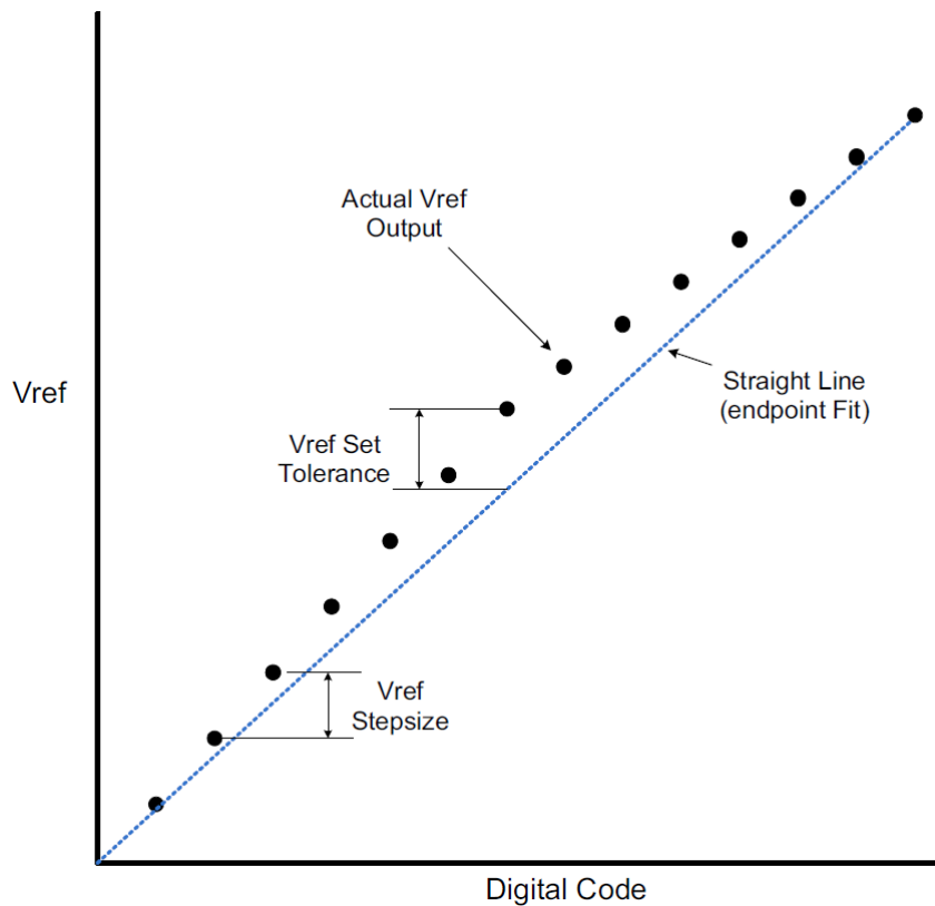
Figure 80: Example of V_{REF} set tolerance (max case only shown) and stepsize
