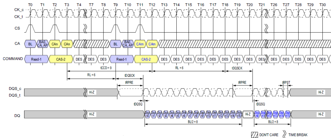
Figure 26: Consecutive Reads Operation: t_{CCD} = \text{Min} + 1 , Preamble = Static, 0.5nCK Postamble
