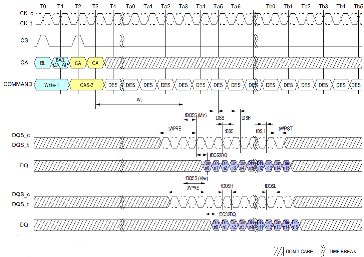
Figure 19: Write Timing
