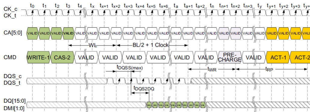
Figure 51: Burst WRITE Followed by PRECHARGE (Shown with BL16, 2tCK pre-amble)
