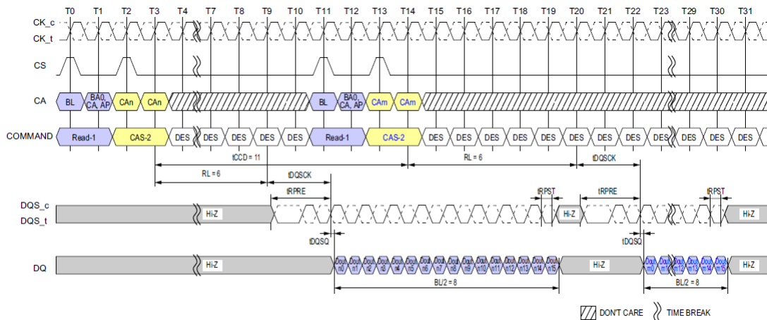
Figure 32: Consecutive Reads Operation: t_{CCD} = \text{Min} + 3 , Preamble = Toggle, 0.5nCK Postamble
