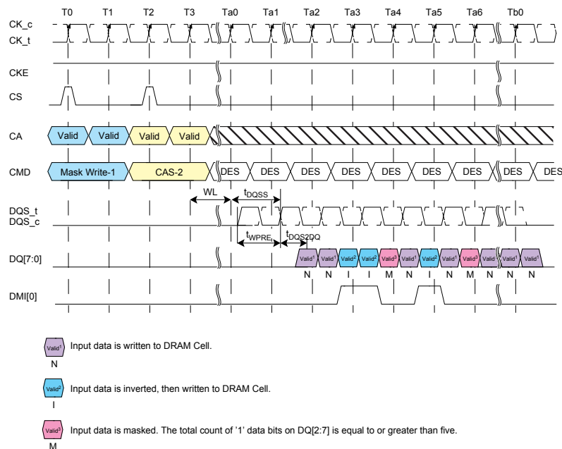
Figure 47: Masked Write Command w/ Write DBI Enabled; DM Enabled
