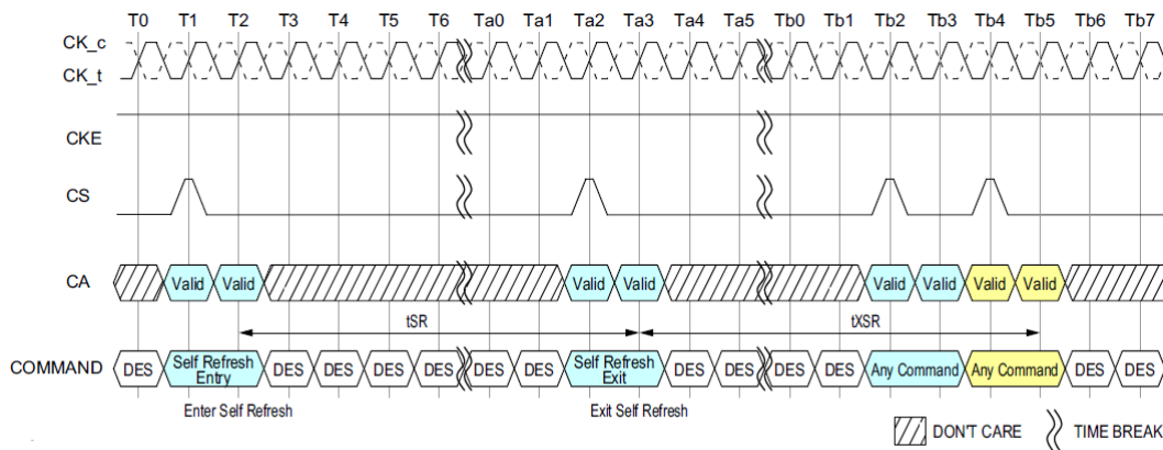
Figure 59: Self Refresh Entry/Exit Timing
