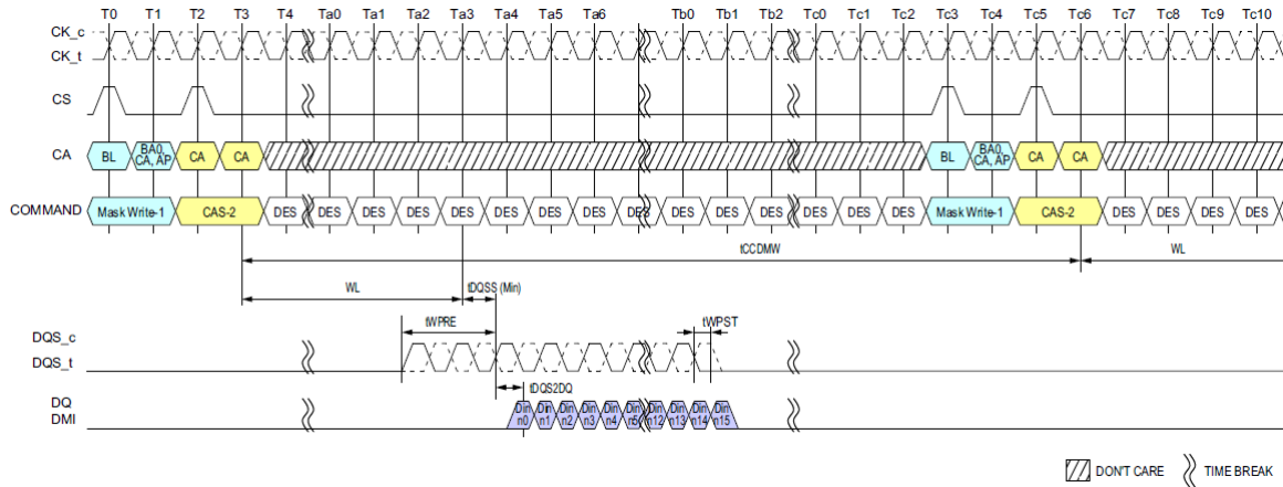
Figure 45: Masked Write Command - Same Bank
