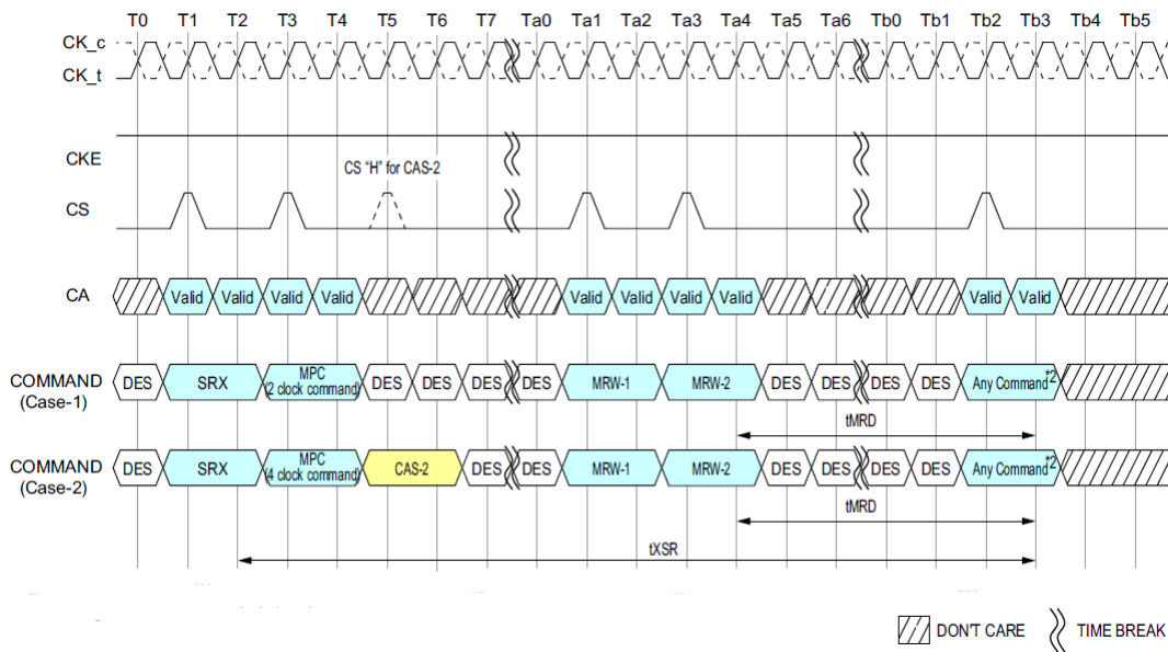
Figure 63: MRR, MRW and MPC Commands Issuing Timing during t_{XSR}
