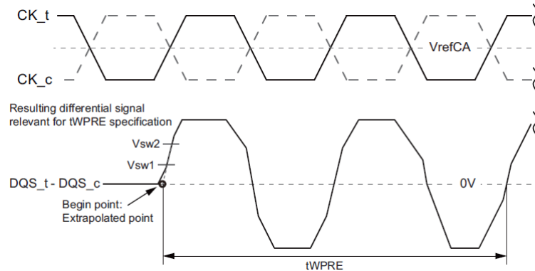
Figure 20: Method for calculating t_{WPRE} transitions and endpoints
