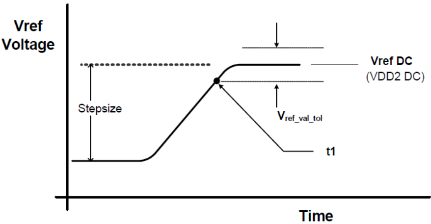
Figure 75: Vref step single stepsize increment case.
