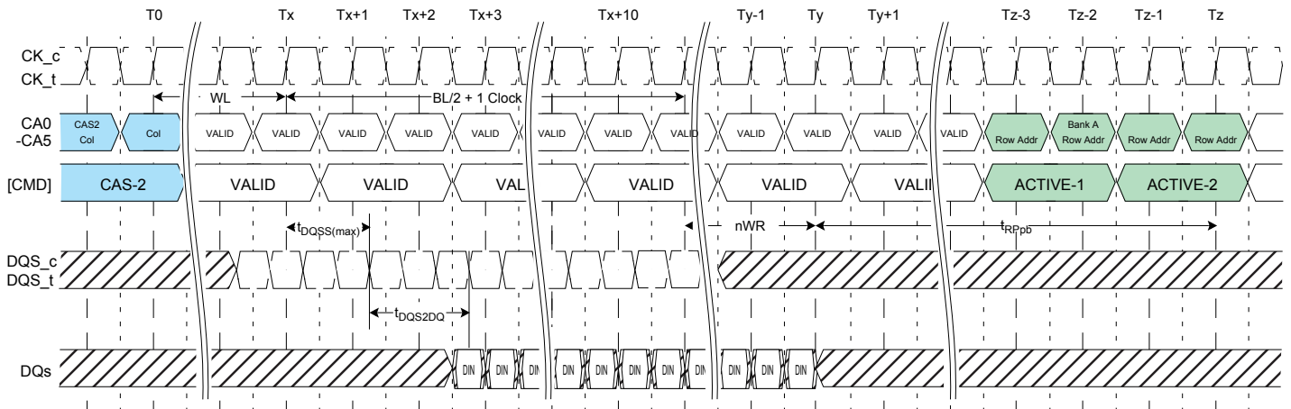
Figure 54: Burst WRITE with Auto Precharge (Shown with BL16, 2tCK pre-ambler)
