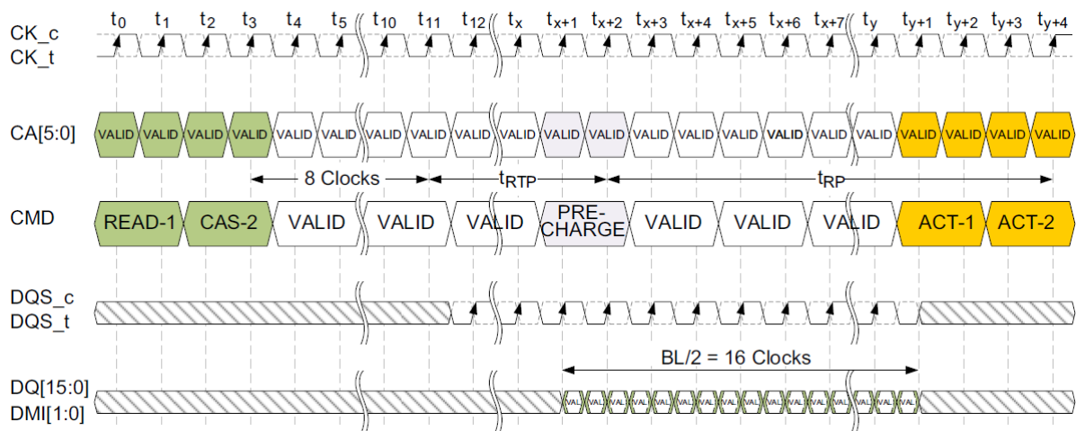
Figure 50: Burst READ followed by PRECHARGE (Shown with BL32, 2tCK pre-ambles)
