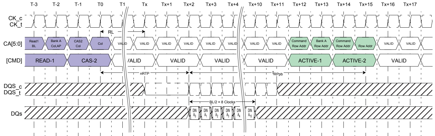
Figure 52: Burst READ with Auto-Precharge (Shown with BL16, 2tCK pre-ample)
