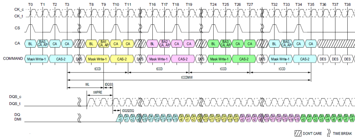
Figure 46: Masked Write Command - Different Bank
