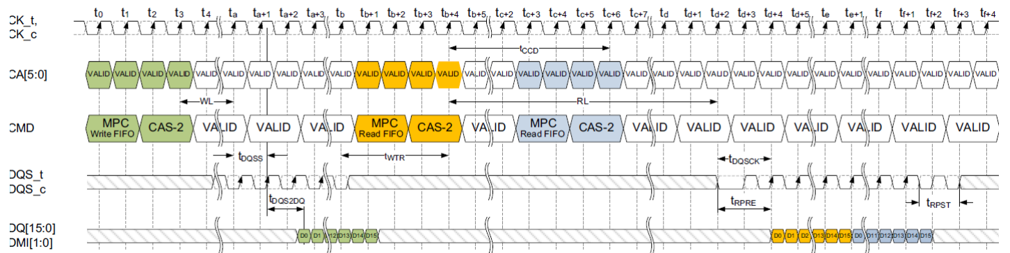
Figure 111: MPC [RD FIFO] Read Operation: t_{WPST}=2nCK , t_{WPST}=0.5nCK , t_{RPST}=toggling , t_{RPST}=1.5nCK
