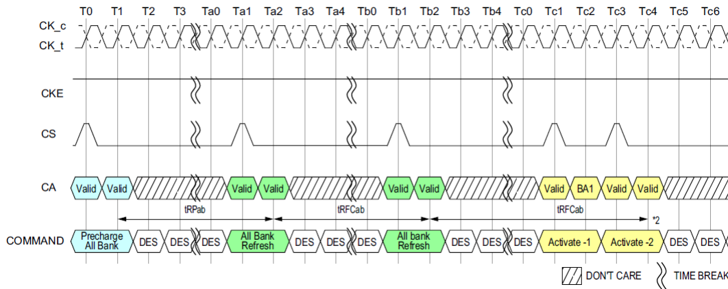
Figure 55: All-Bank Refresh Operation
