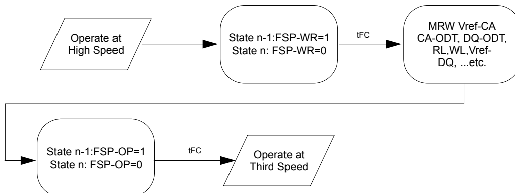
Figure 93: Switching to a Third Trained Frequency Set-Point
