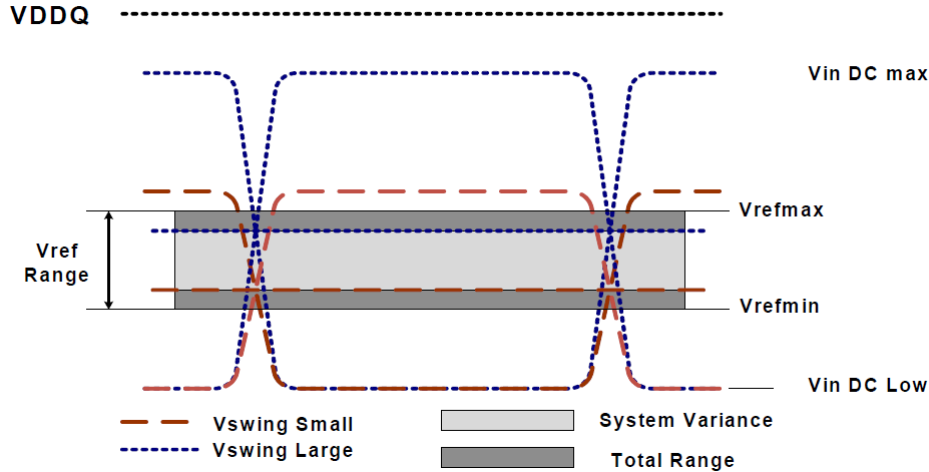
Figure 79: V_{REF} operating range( V_{REFmin} , V_{REFmax} )
