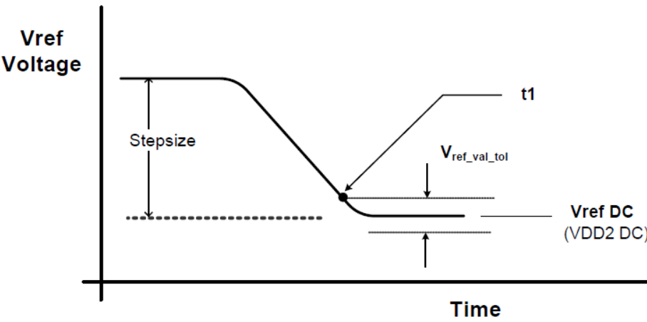
Figure 76: Vref step single stepsize decrement case
