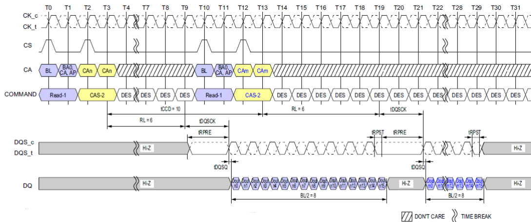
Figure 30: Consecutive Reads Operation: t_{CCD} = \text{Min} +2 , Preamble = Static, 0.5nCK Postamble
