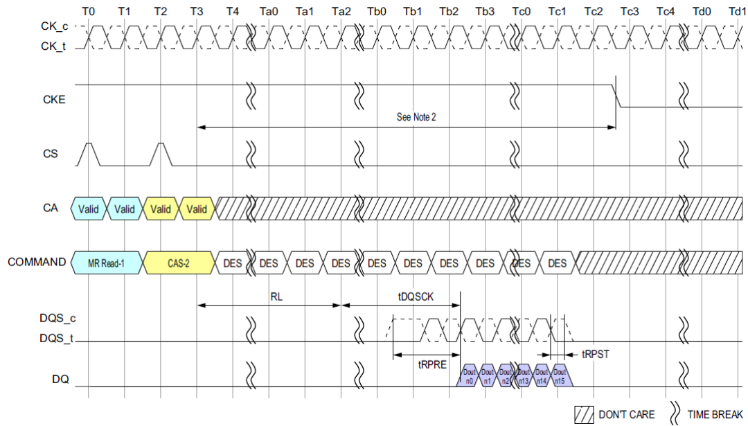
Figure 131: Mode Register Read to Power-Down Entry
