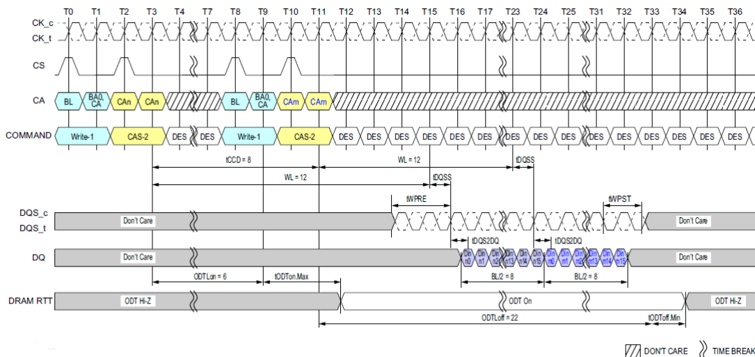
Figure 36: Seamless Writes Operation: t_{CCD} = \text{Min} , 1.5nCK Postamble, 533MHz < Clock Freq. ≤ 800MHz, ODT Worst Timing Case
