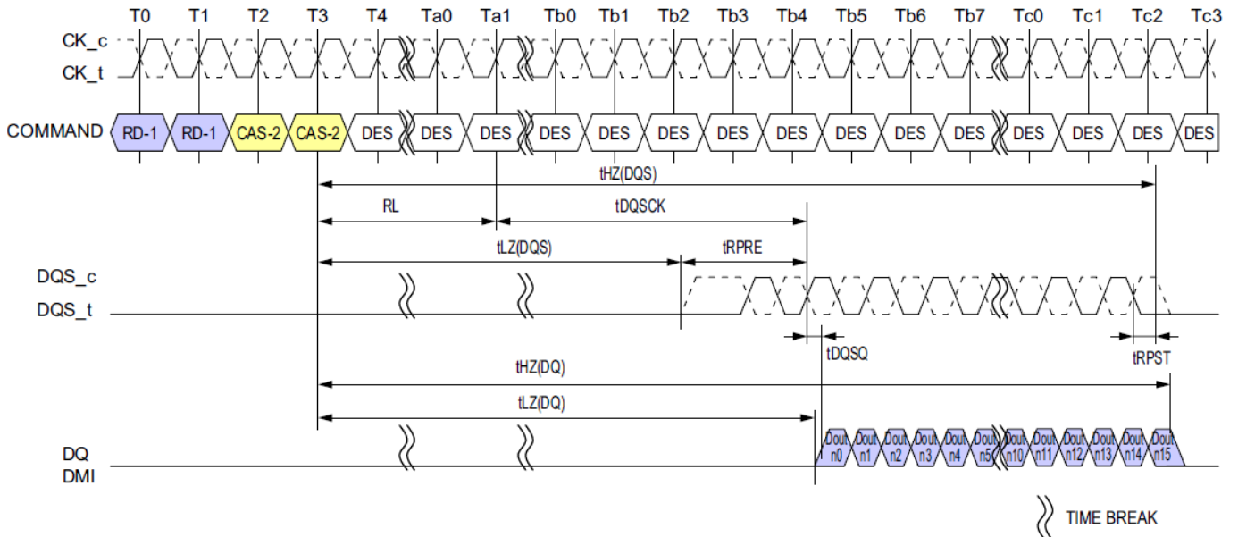
Figure 10: Read Timing
