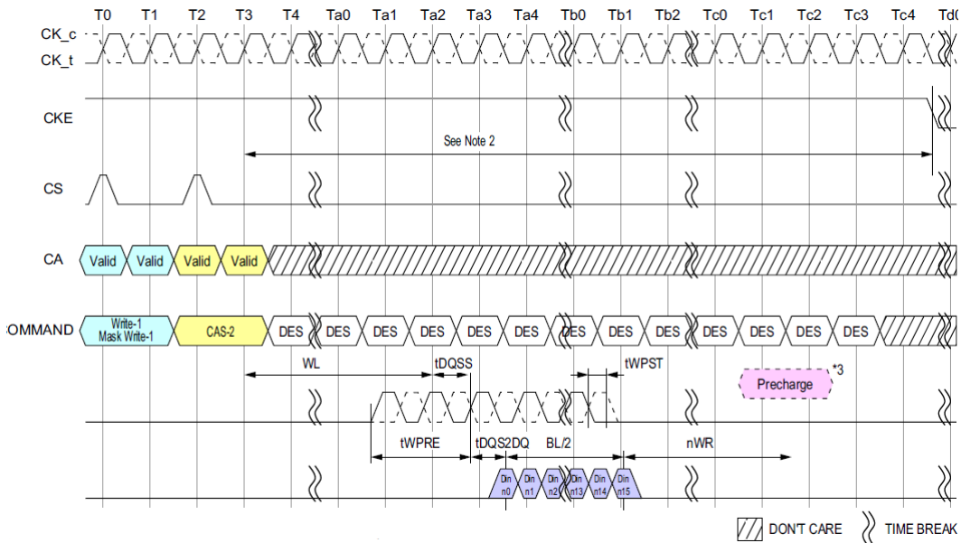
Figure 127: Write with Auto Precharge and Mask Write with Auto Precharge to Power-Down Entry
