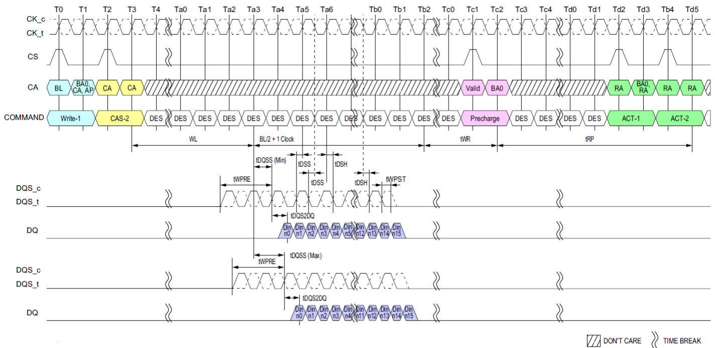
Figure 17: Burst Write Operation
