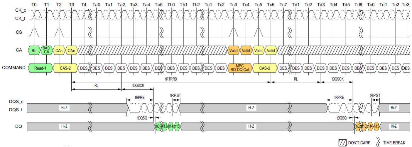
Figure 98: DQ Read Training Timing: Read to Read DQ Calibration
