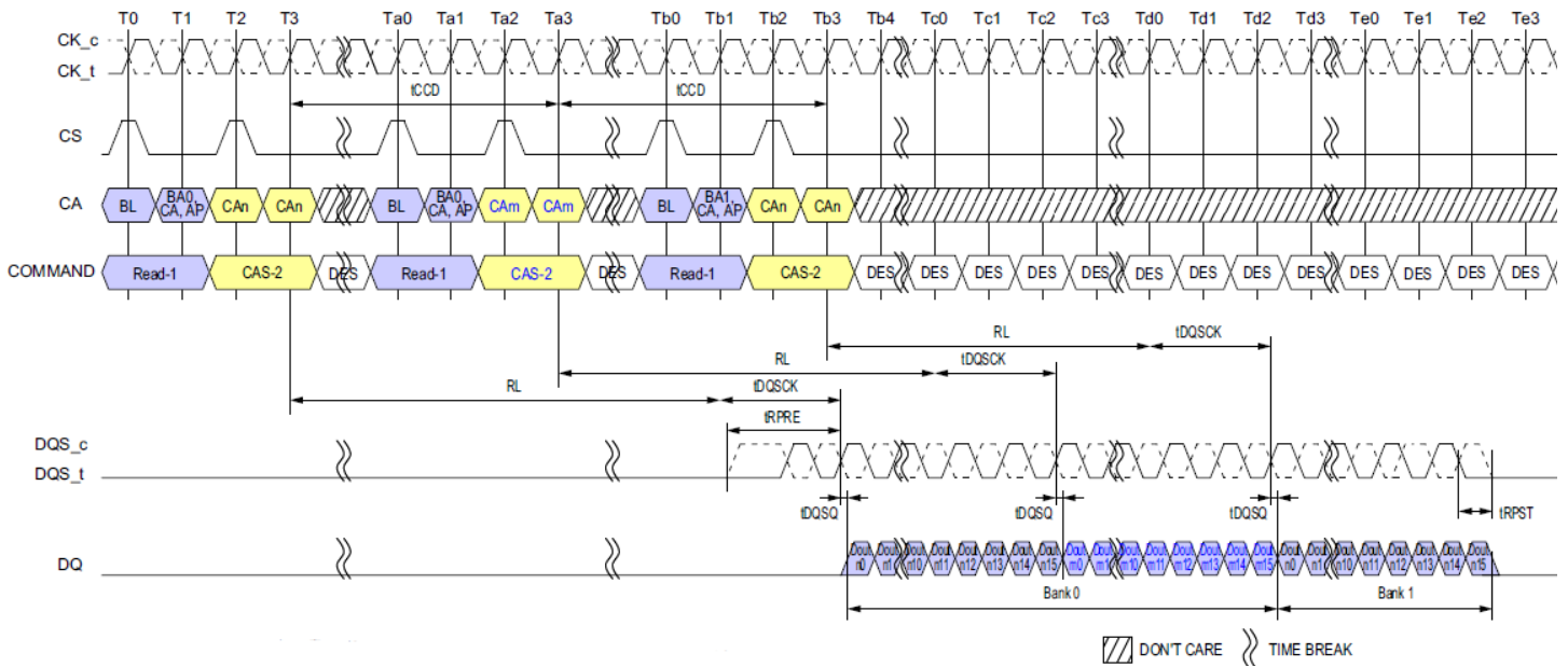
Figure 9: Seamless Burst Read
