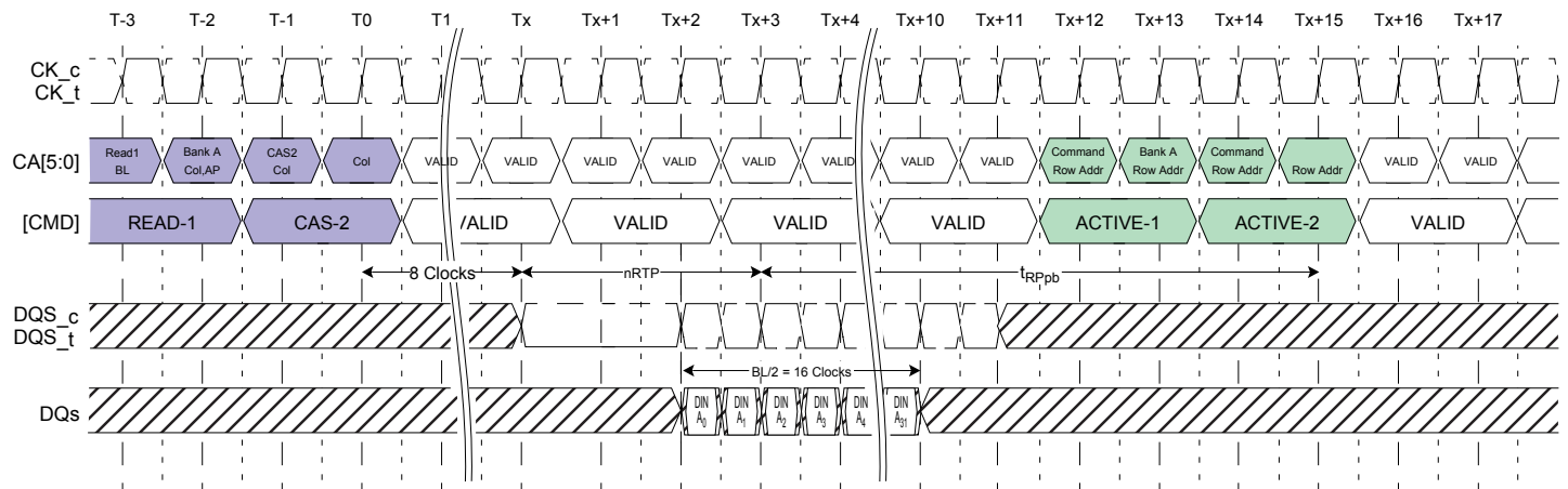
Figure 53: Burst READ with Auto-Precharge (Shown with BL32, 2tCK pre-ample)
