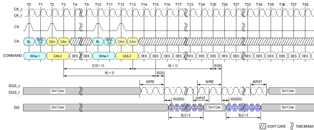
Figure 41: Consecutive Writes Operation: t_{CCD} = \text{Min} + 2, 1.5nCK Postamble
