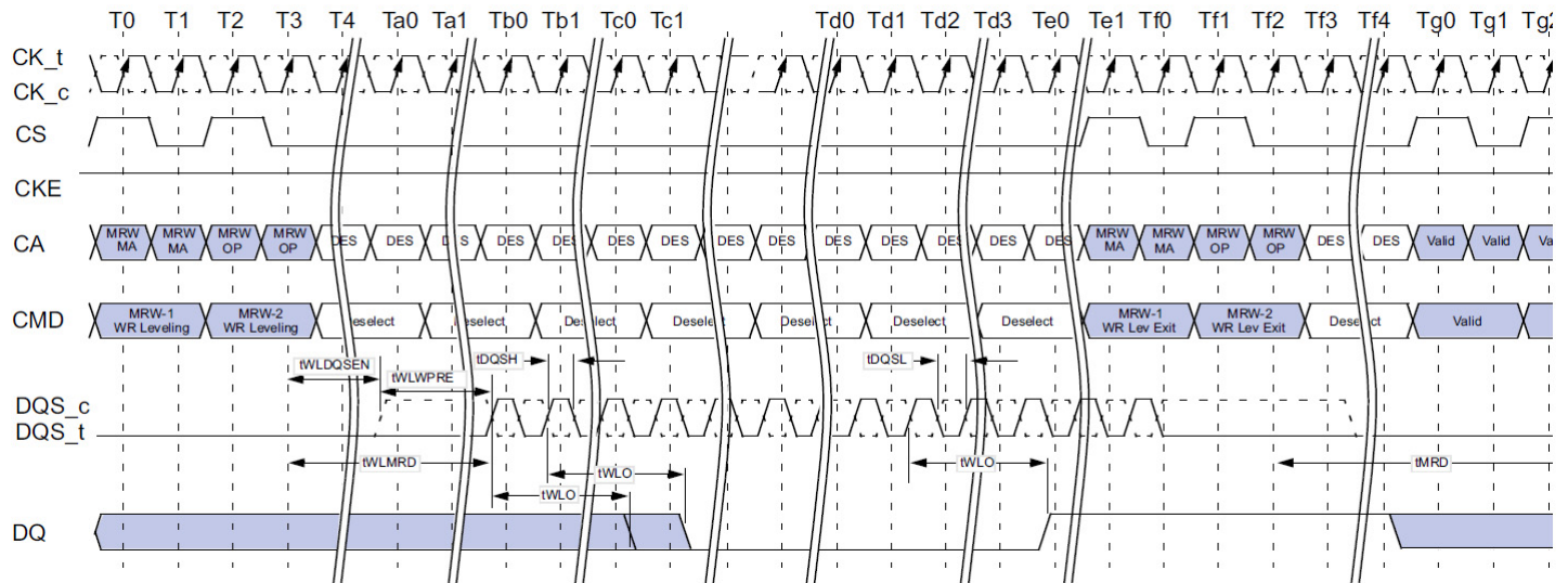
Figure 95: Write Leveling Timing, t_{DQSL(min)}
