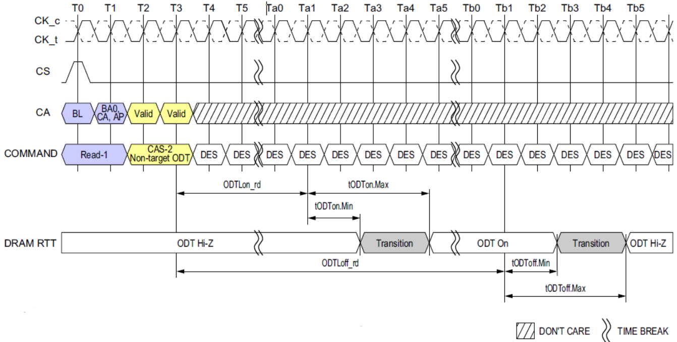
Figure 122: ODT Control on Non-target DRAM for Read
