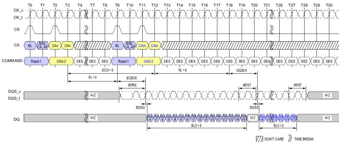
Figure 23: Consecutive Reads Operation: t_{CCD} = \text{Min} + 1 , Preamble = Toggle, 1.5nCK Postamble
