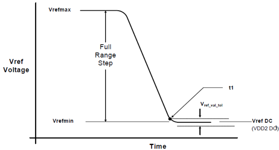
Figure 78: Vref full step from Vrefmax to Vrefmin case.
