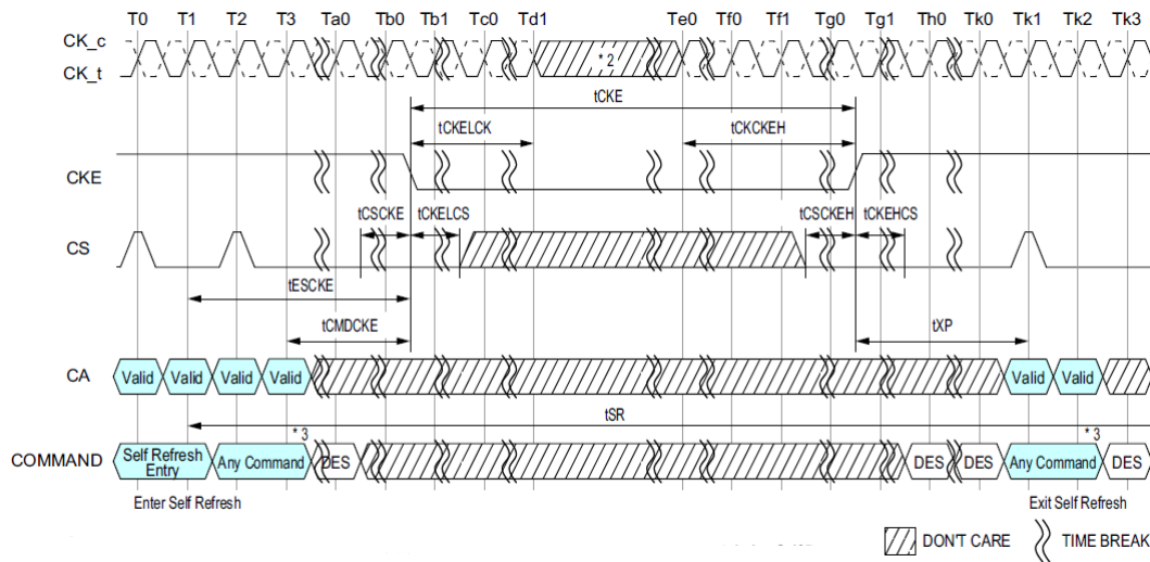
Figure 61: Command input timings after Power Down Exit during Self Refresh
