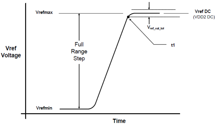
Figure 77: Vref full step from Vrefmin to Vrefmax case
