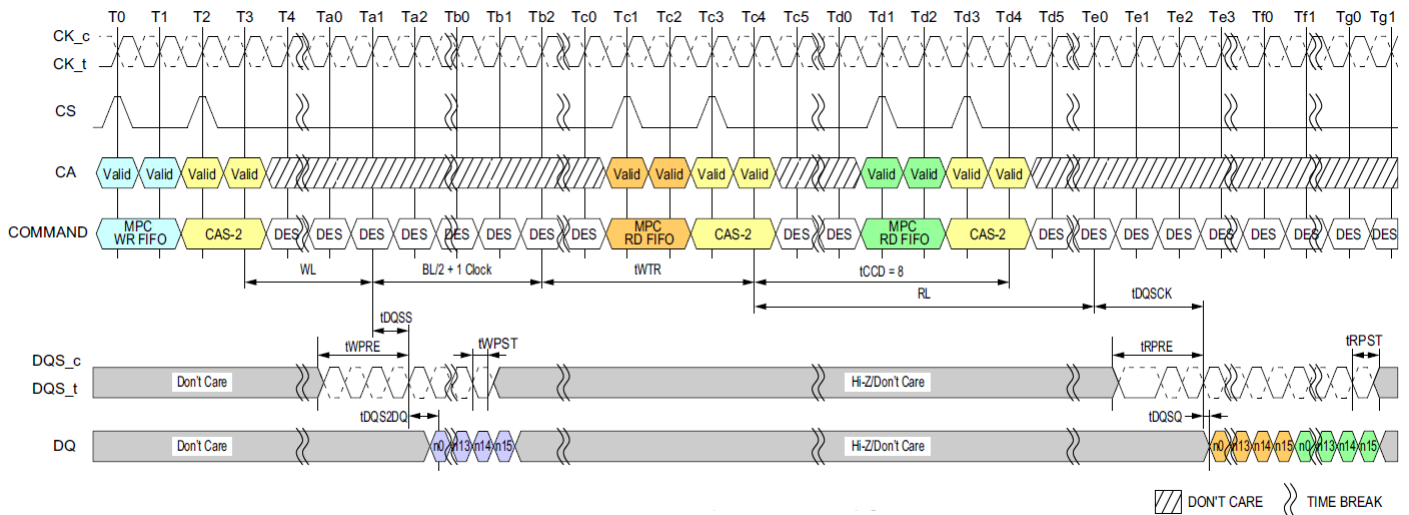
Figure 102: MPC [Write FIFO] to MPC [Read FIFO] Timing
