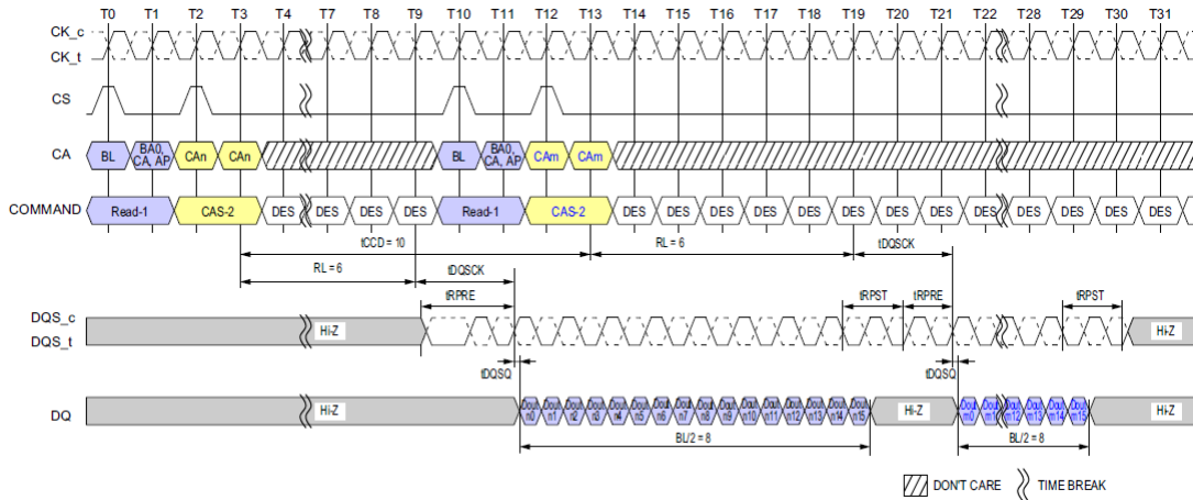
Figure 27: Consecutive Reads Operation: t_{CCD} = \text{Min} + 2 , Preamble = Toggle, 1.5nCK Postamble
