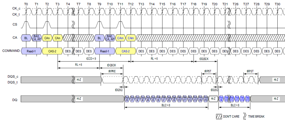
Figure 25: Consecutive Reads Operation: t_{CCD} = \text{Min} + 1 , Preamble = Static, 1.5nCK Postamble
