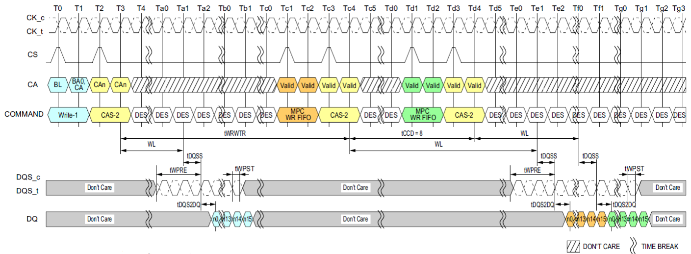
Figure 101: Write to MPC [Write FIFO] Operation Timing
