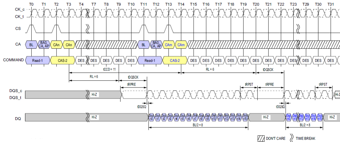
Figure 33: Consecutive Reads Operation: t_{CCD} = \text{Min} + 3 , Preamble = Static, 1.5nCK Postamble
