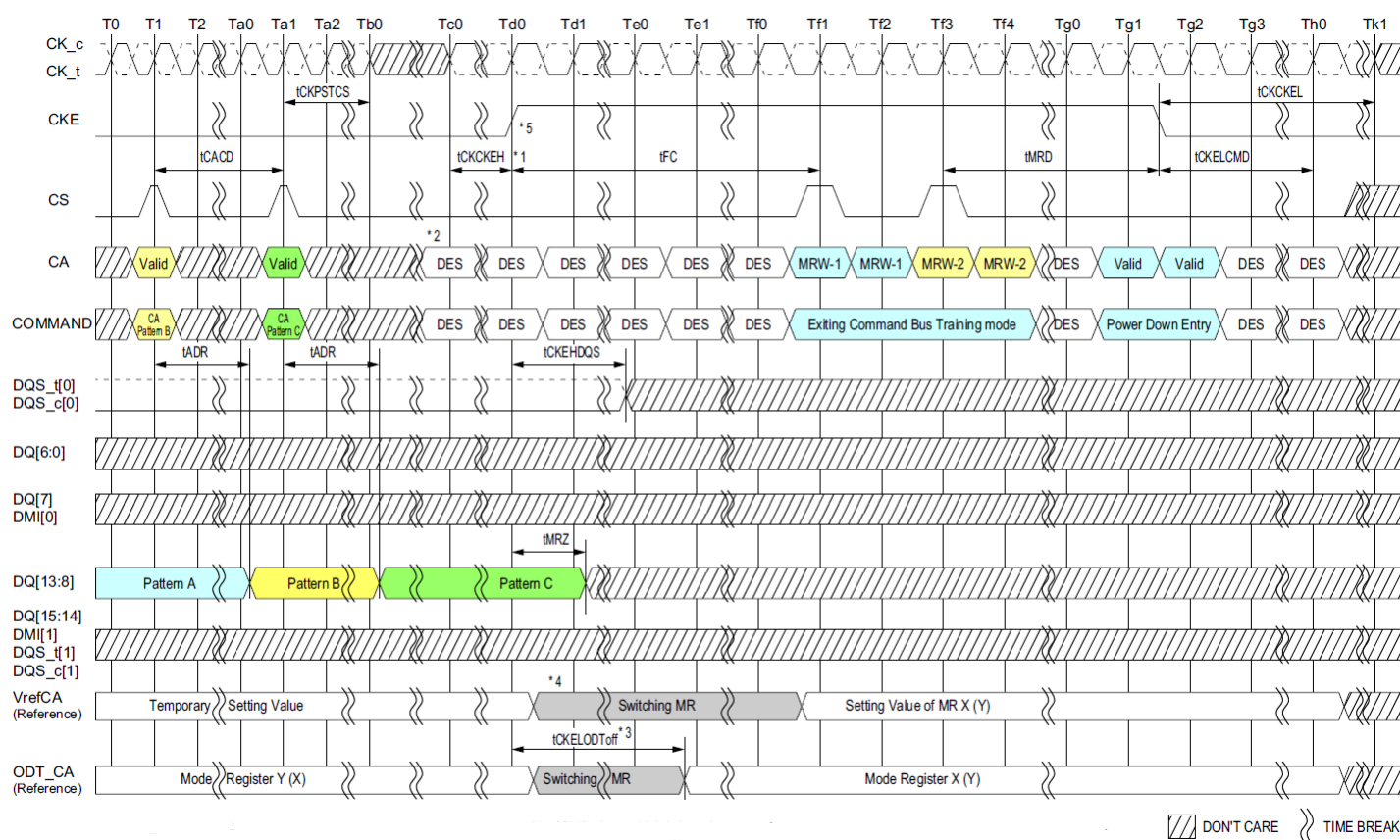
Figure 89: Exiting Command Bus Training Mode with Power Down Entry
