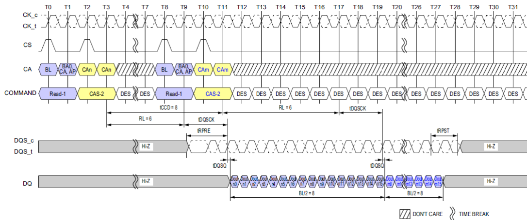
Figure 22: Seamless Reads Operation: t_{CCD} = \text{Min} , Preamble = Toggle, 1.5nCK Postamble
