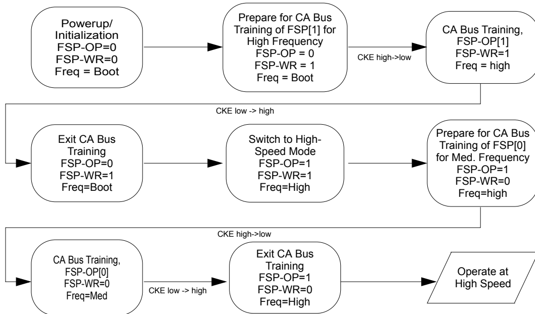
Figure 91: Training Two Frequency Set-Points
