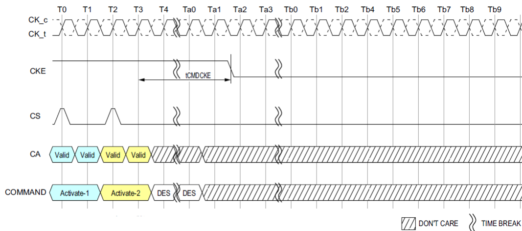
Figure 129: Activate Command to Power-Down Entry
