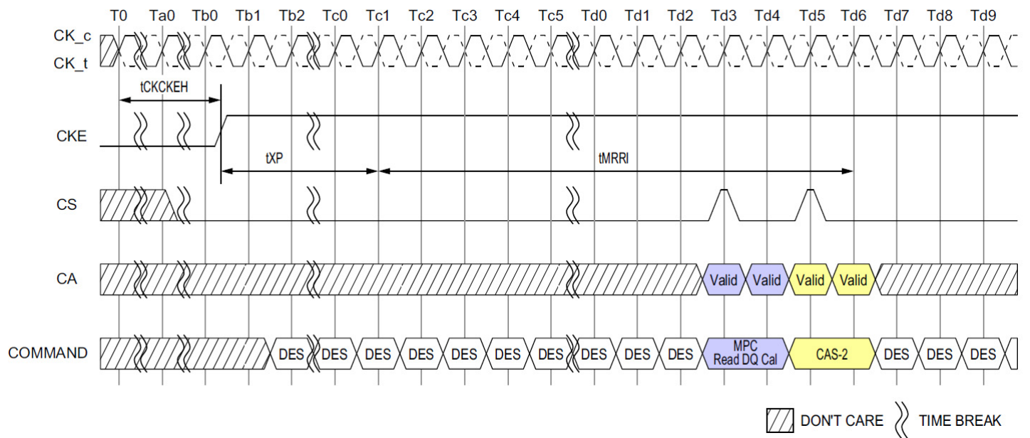
Figure 100: MPC Read DQ Calibration Following Power-Down State
