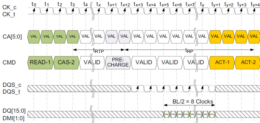
Figure 49: Burst READ Followed by PRECHARGE (Shown with BL16, 2tCK pre-ambles)
