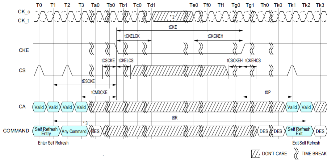
Figure 60: Self Refresh Entry/Exit Timing with Power Down Entry/Exit
