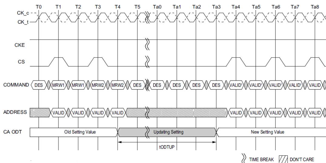
Figure 117: ODT for Command/Address setting update timing in 4 Clock Cycle Command
