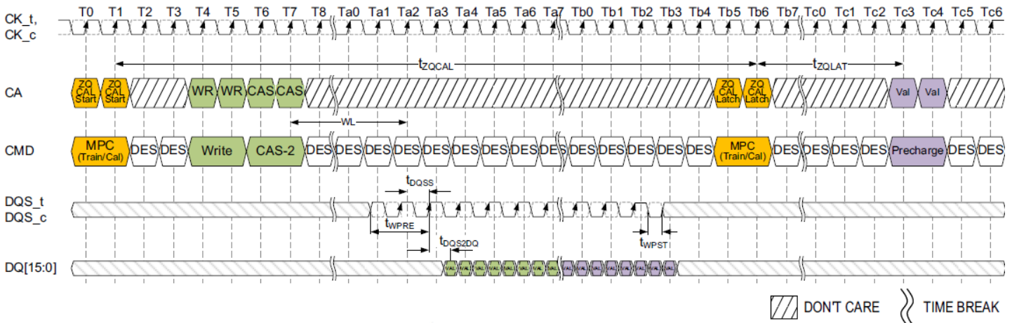
Figure 114: ZQCal Timing
