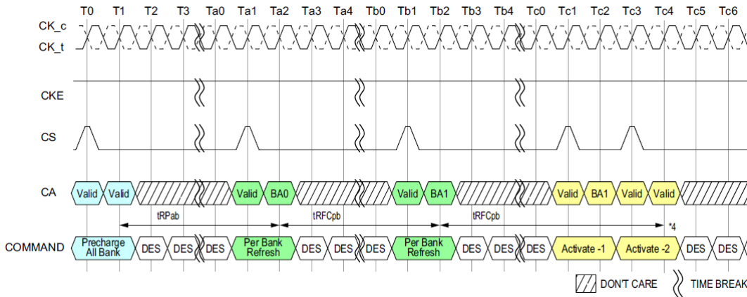
Figure 56: Per-Bank Refresh Operation
