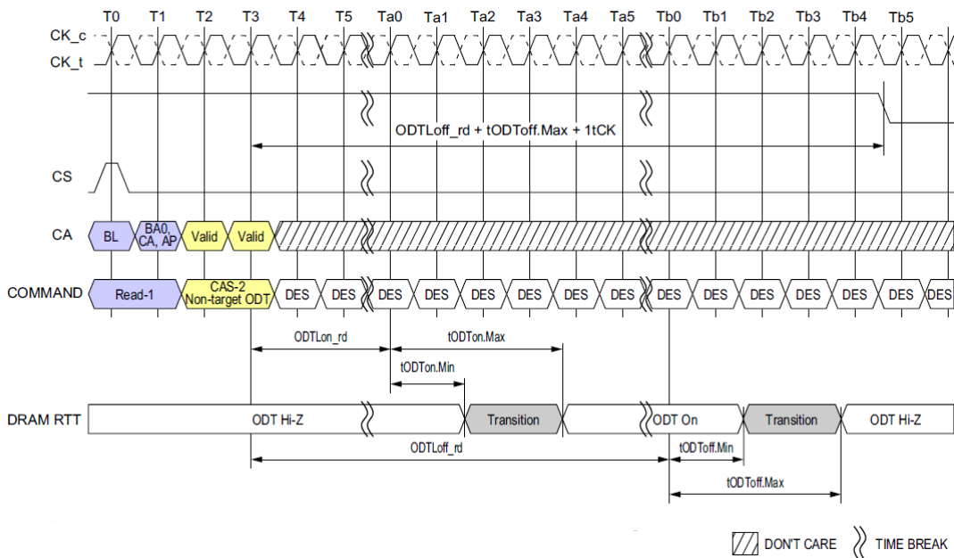
Figure 123: Non-target DRAM for Read to Power-Down Entry
