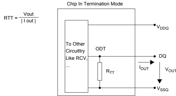
Figure 120: On Die Termination
