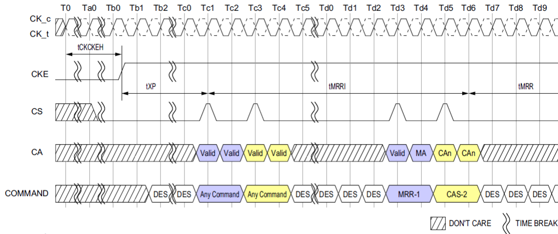
Figure 68: MRR Following Power-Down
