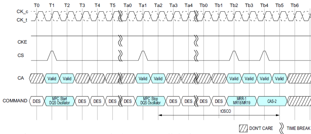
Figure 107: In case of DQS Interval Oscillator is stopped by MPC Command
