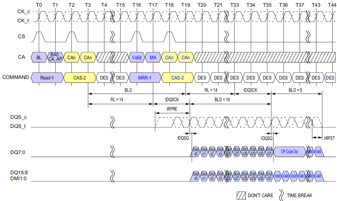
Figure 66: READ to MRR Timing
