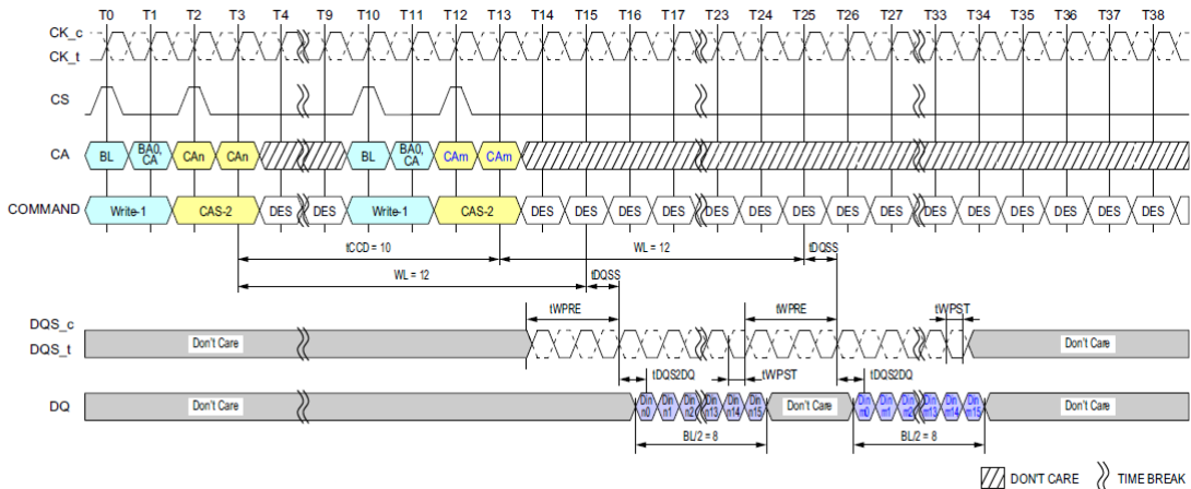
Figure 40: Consecutive Writes Operation: t_{CCD} = \text{Min} + 2, 0.5nCK Postamble
