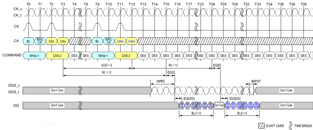
Figure 38: Consecutive Writes Operation: t_{CCD} = \text{Min} + 1, 0.5nCK Postamble
