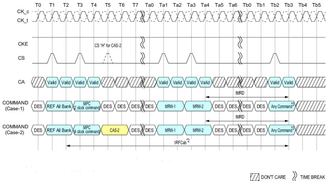
Figure 64: MRR, MRW and MPC Commands Issuing Timing during t_{RFC}
