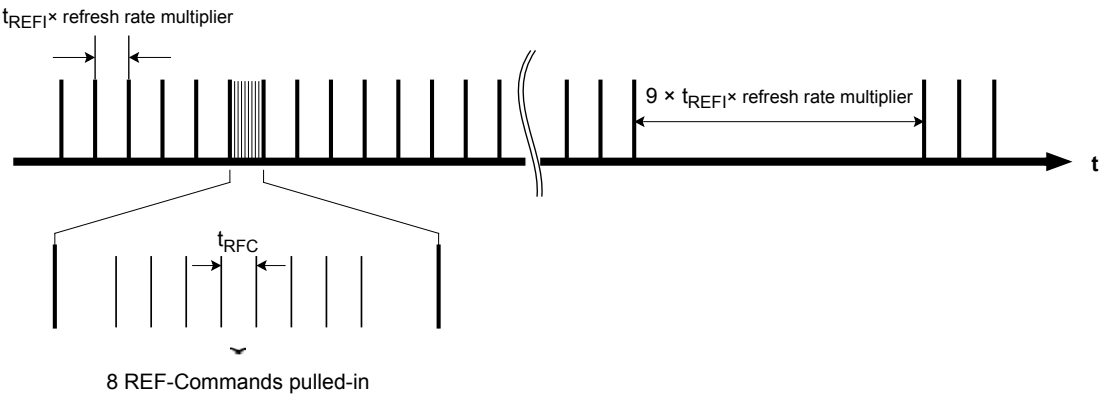
Figure 58: Pulling-in Refresh Commands (Example)
