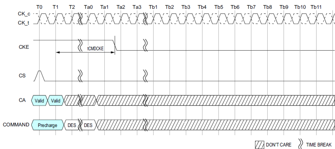
Figure 130: Precharge Command to Power-Down Entry
