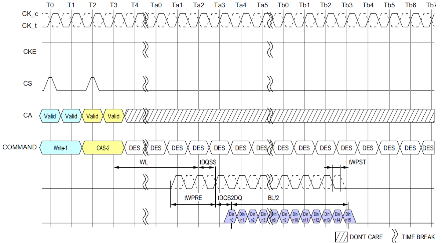
Figure 15: DQS Write Preamble and Postamble: 0.5nCK Postamble
