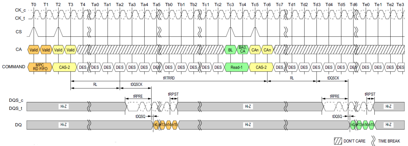
Figure 103: MPC [Read FIFO] to Read Timing
